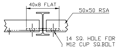
SECTION THRU POST
