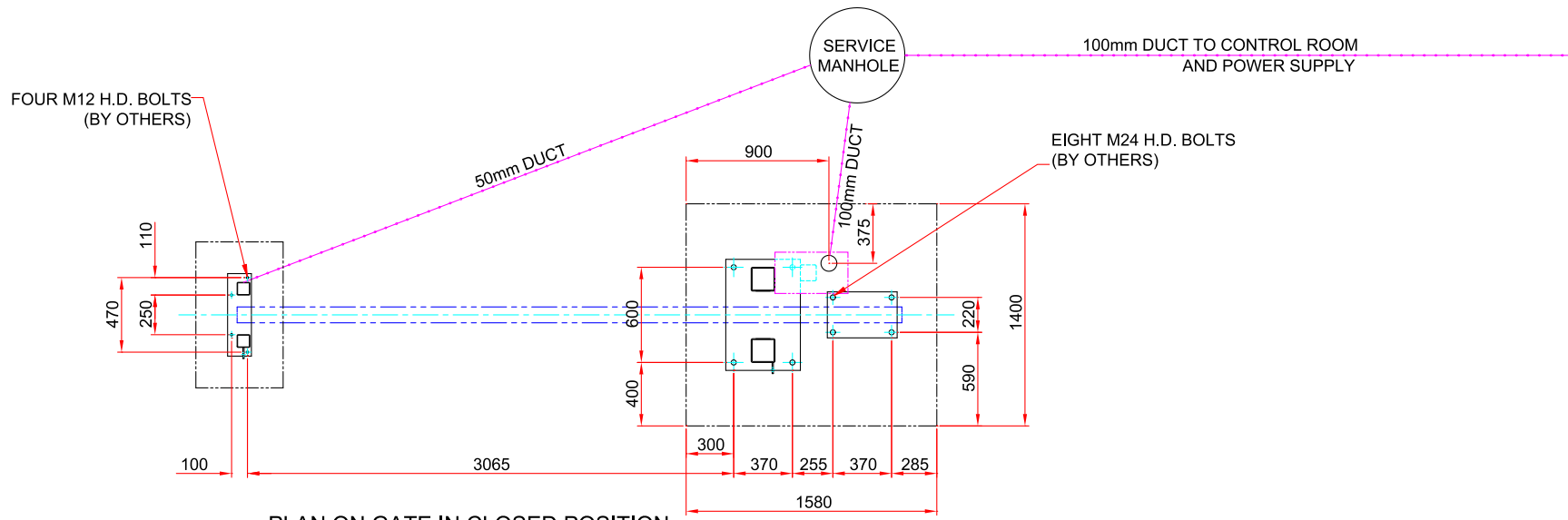
PLAN ON GATE IN CLOSED POSITION
