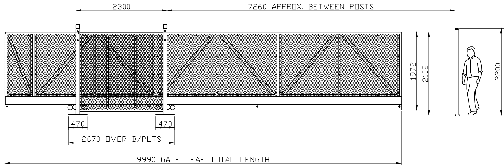
Heavy Duty 7m wide fully automatic gate, closes to right General arrangement
