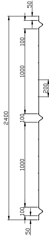
SECTION - 2.4m HIGH PANEL
