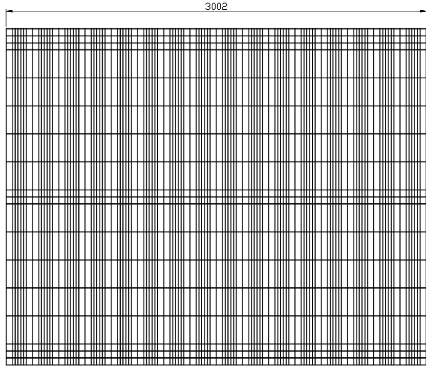
ELEVATION - 2.4m HIGH PANEL
