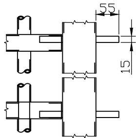
FIXING DETAIL
